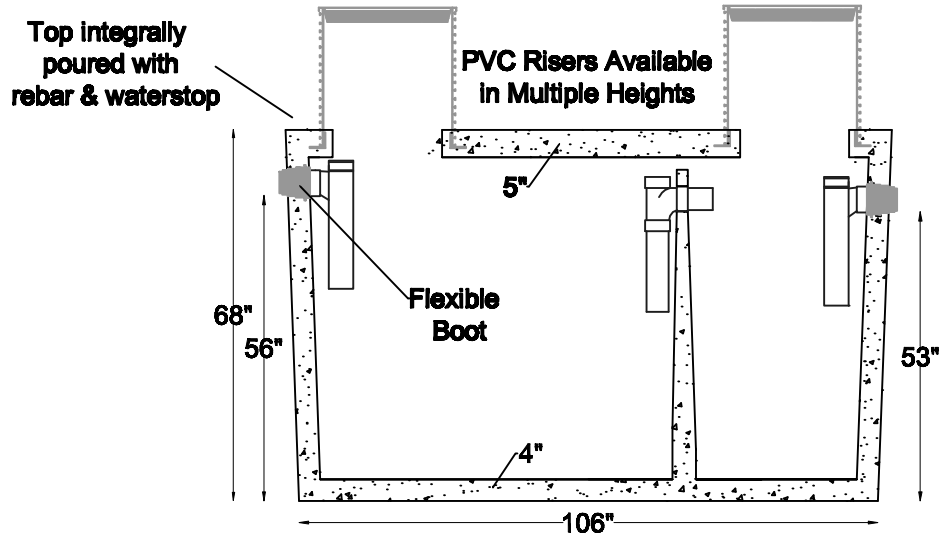
Section View
