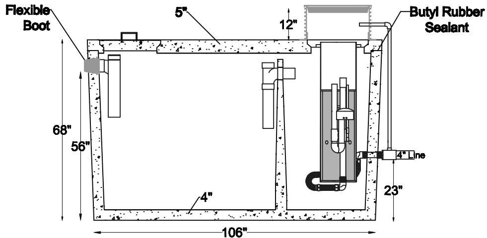
Section View
