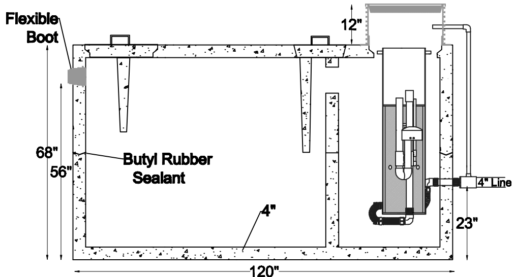
Section View
