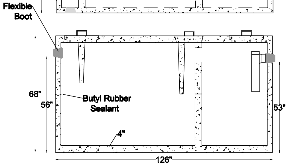
Section View
