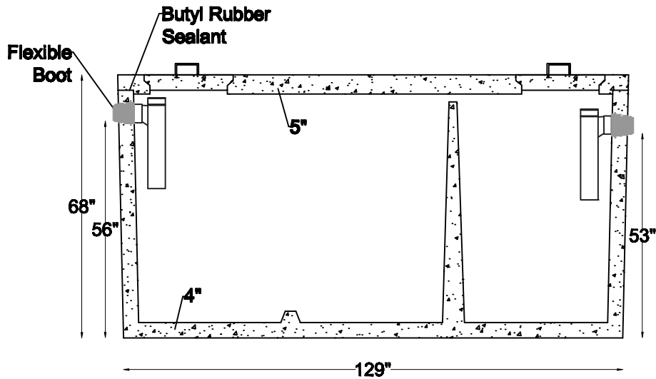
Section View
