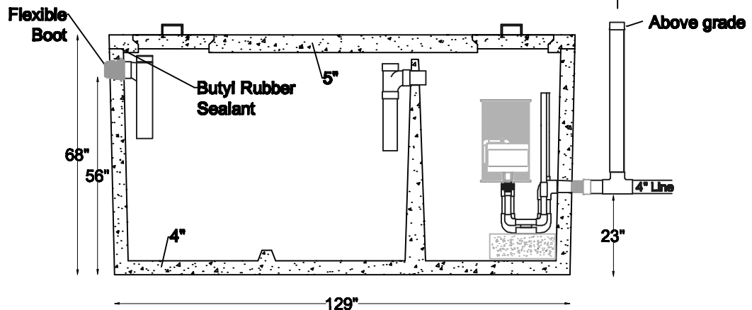
Section View
