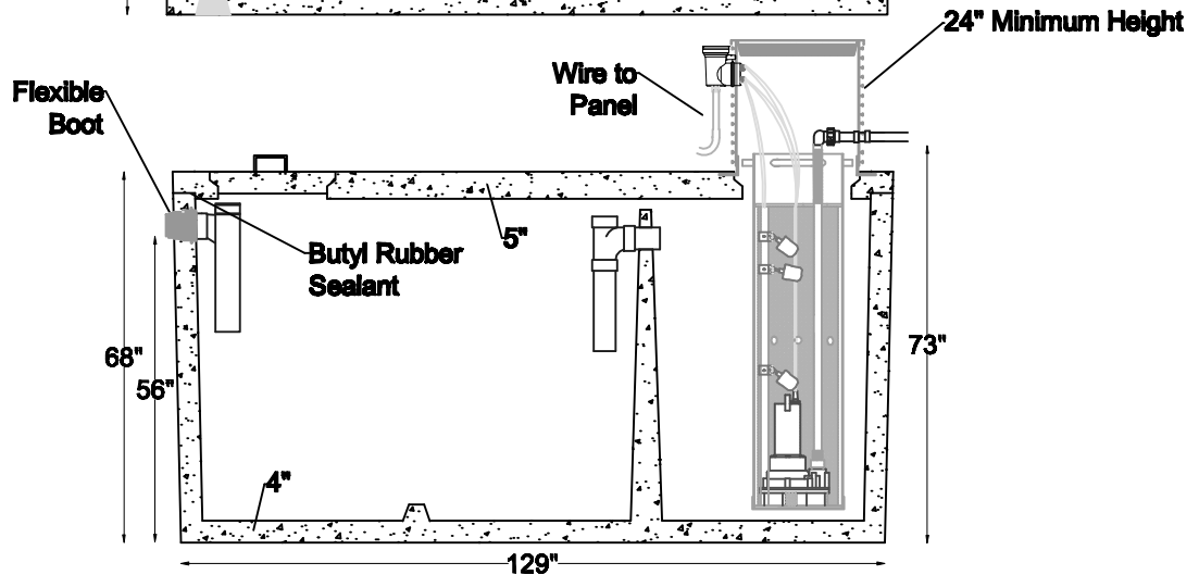
Section View
