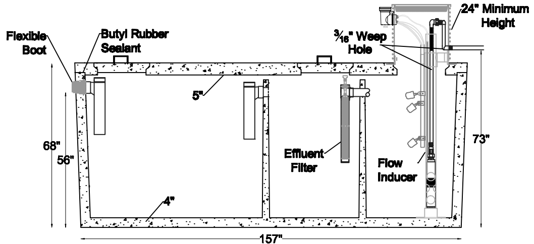
Section View
