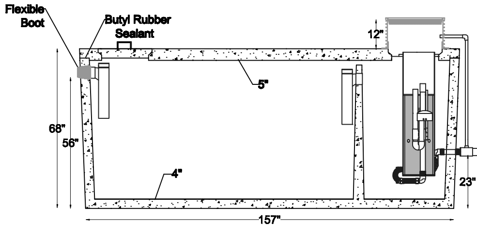
Section View
