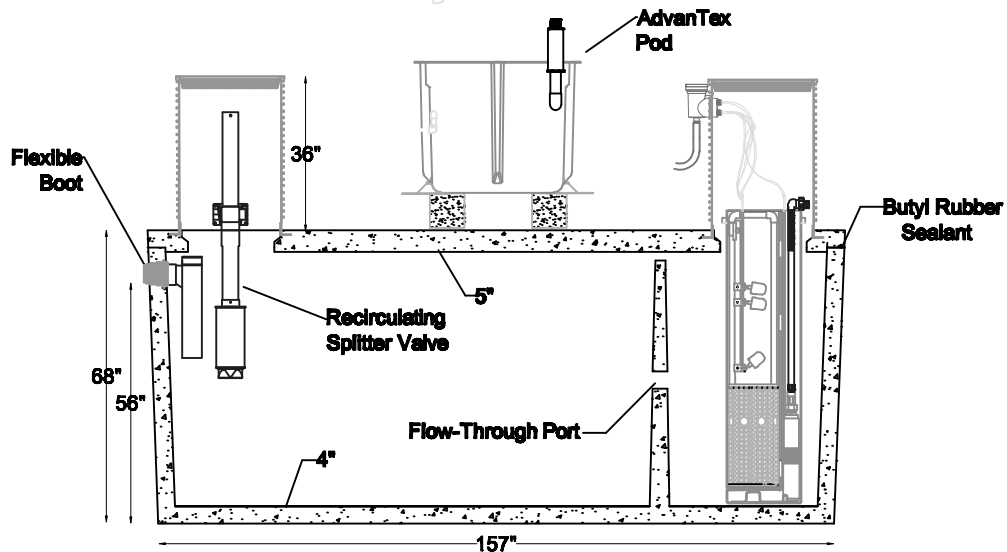
Section View
